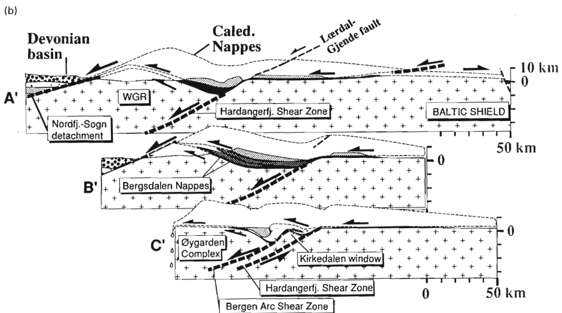
Fig. 1. (a) Simplified geologic map of southern Norway. HRNC = Hardanger-Ryfylke Nappe Complex. NSD = Nordfjord-Sogn Detachment. (b) Profiles indicated in (a).
