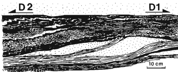
Fig. 13. Structures in mylonite at the base of the Hardanger-Ryfylke Nappe Complex close to the phyllite, Haukelidunellen. Sigmoidal-shaped competent (stippled) lenses in the weak (dark) mylonite indicate top-to-the-southeast sense of shear ( D_1 ). Later asymmetric small-scale folding and a SE-dipping crenulation cleavage is developed in weak, mica-rich layers, indicating post- D_1 reversal of the shear direction. Redrawn from photograph.
