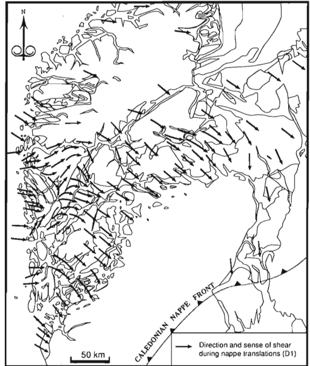
Fig. 4. Shear sense and thrusting directions during the Caledonian contraction ( D_1 ). Data from Kvale (1953), Hossack (1968), Nystuen (1983), Morley (1986), Séguret et al. (1989), and own observations.
